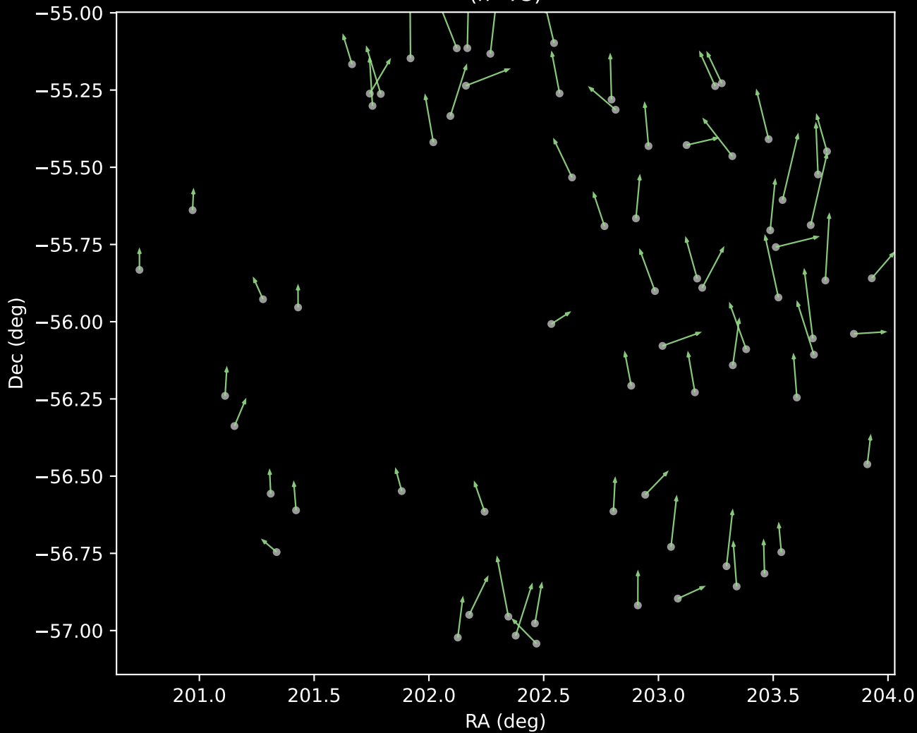
GALAH DR4 Cluster 5 Proper Motion Vectors (n=73)
