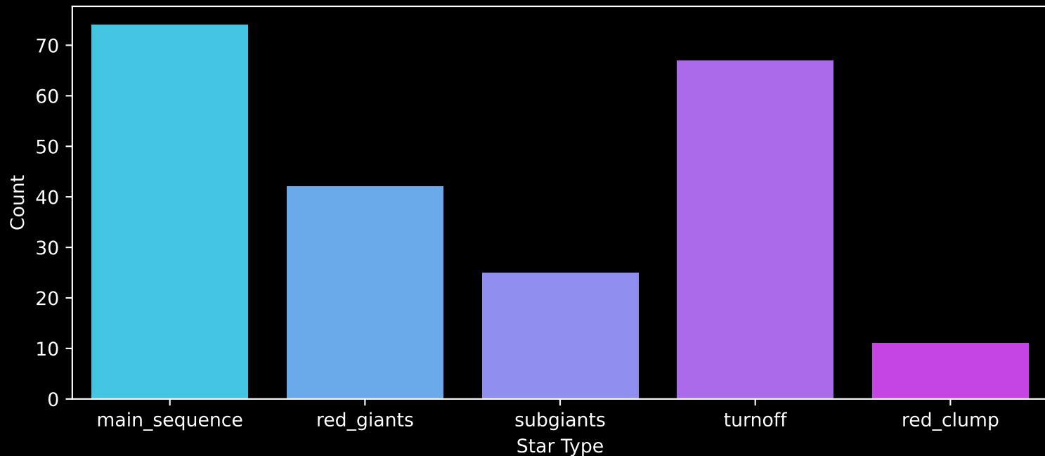
GALAH DR4 Field: [7223] Count plot of Star Type
