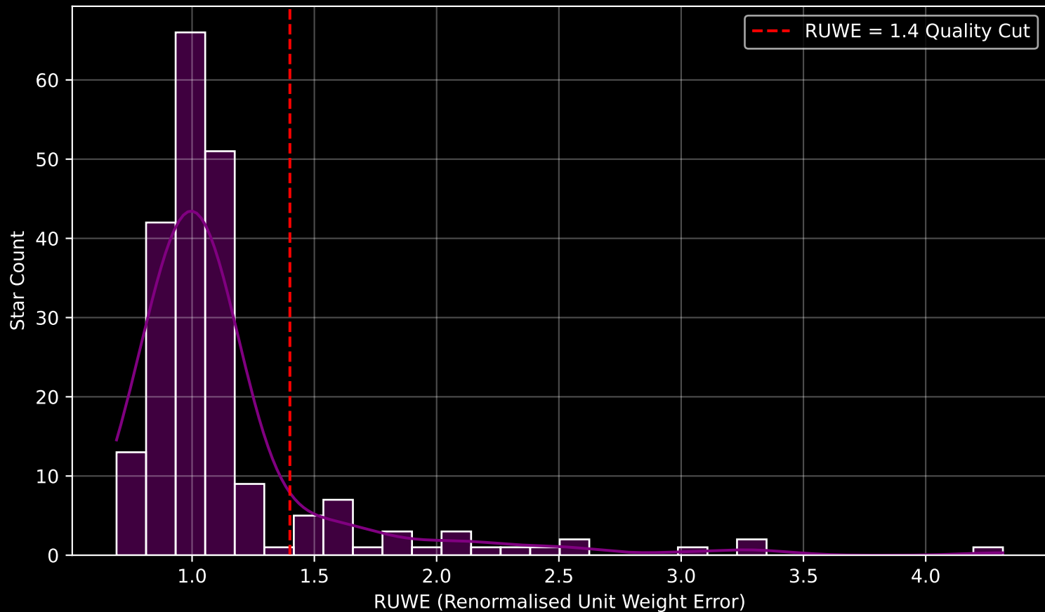
GALAH DR4 Field [7223] RUWE Distribution (n= 211)
