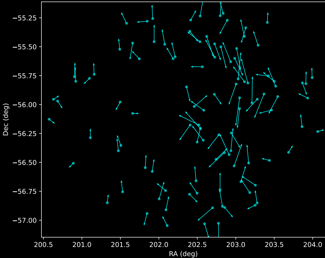
GALAH DR4 Noise Stream Proper Motion Vectors (n=104)
